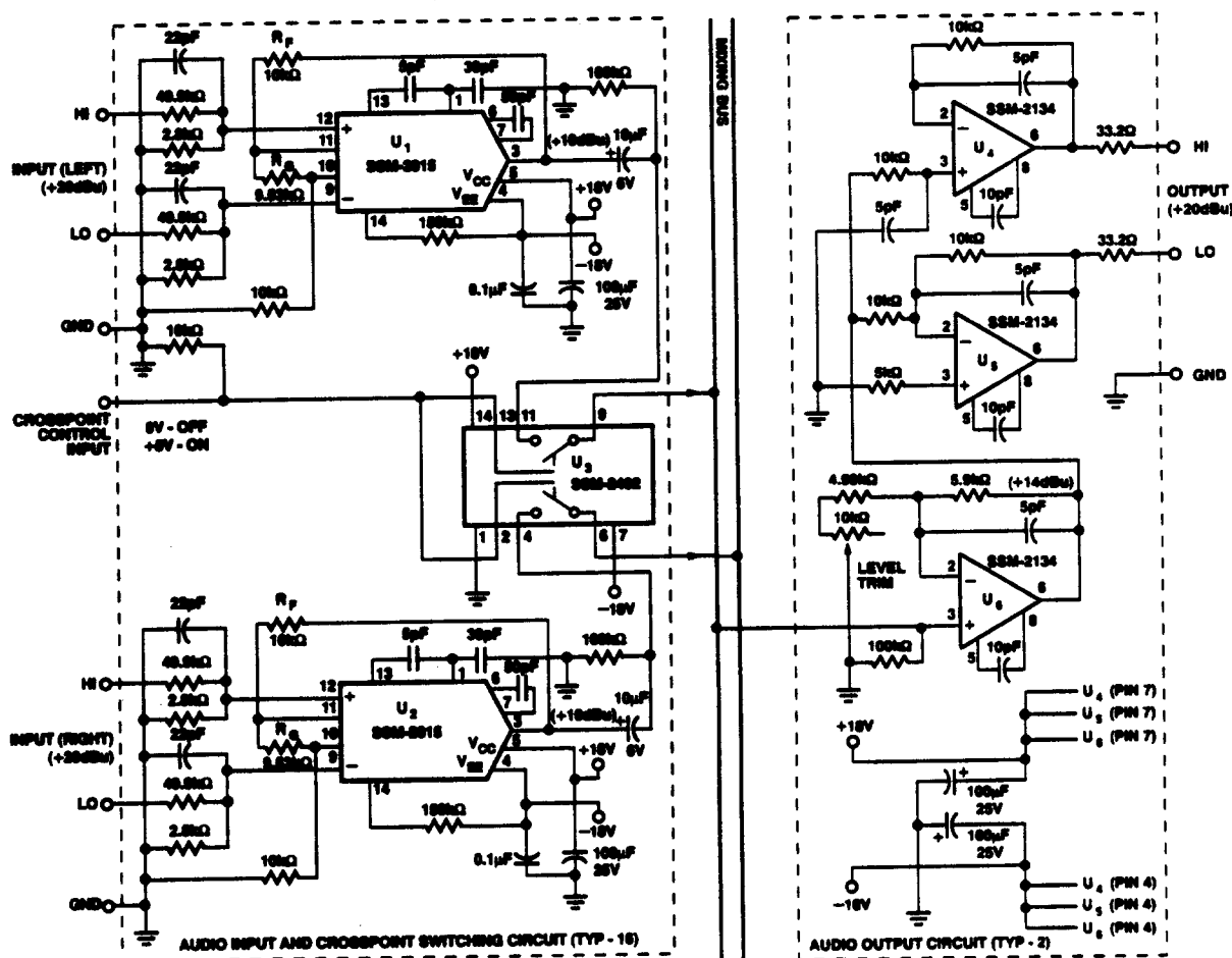
FIGURE 1: Switcher Schematic
